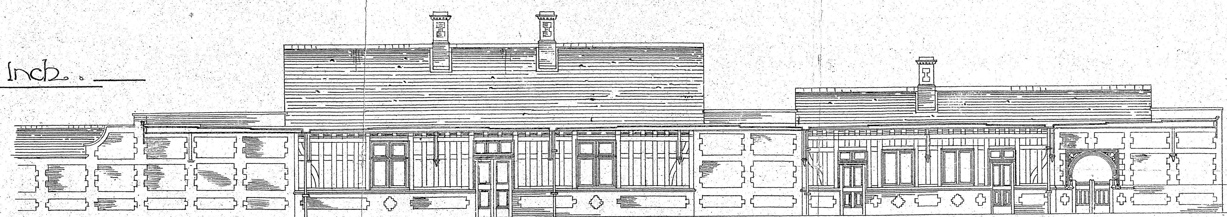
Elevation to Down Platform.
