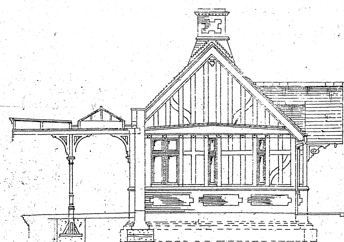
End Elevation B.B.
