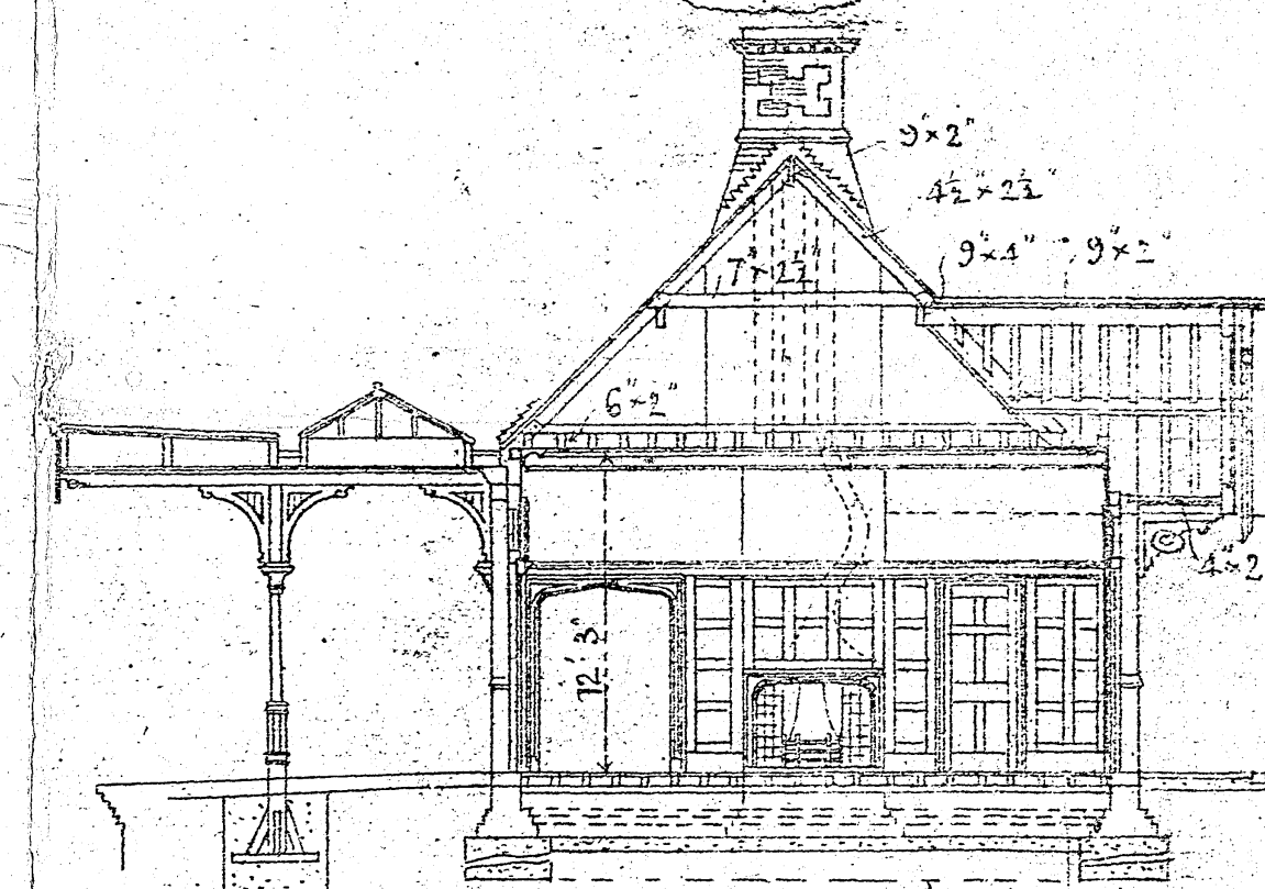
Section C.C.
