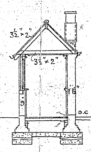
Section thro' Corridor.
